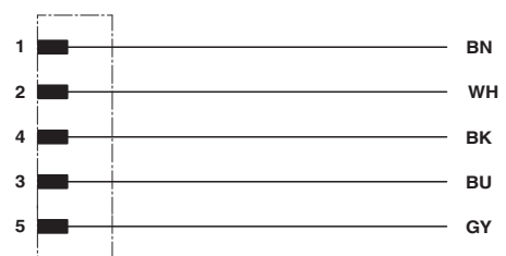
Circuit diagram
